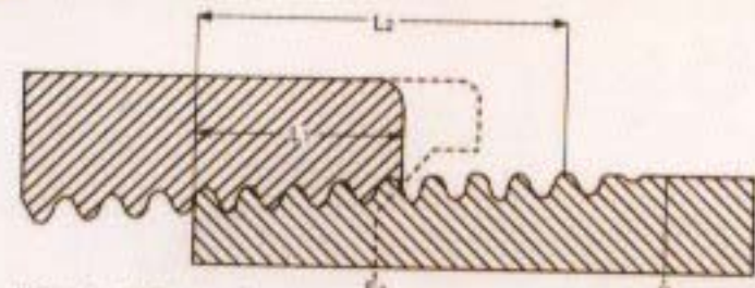
Fig. 5. (Taper) L_2 = (0.8D + 6.8) \times 1/16
