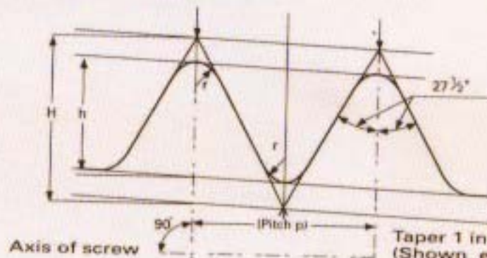
Fig. 2. (Taper) H = 0.960237 \times p h = 0.640327 \times p r = 0.137278 \times p
